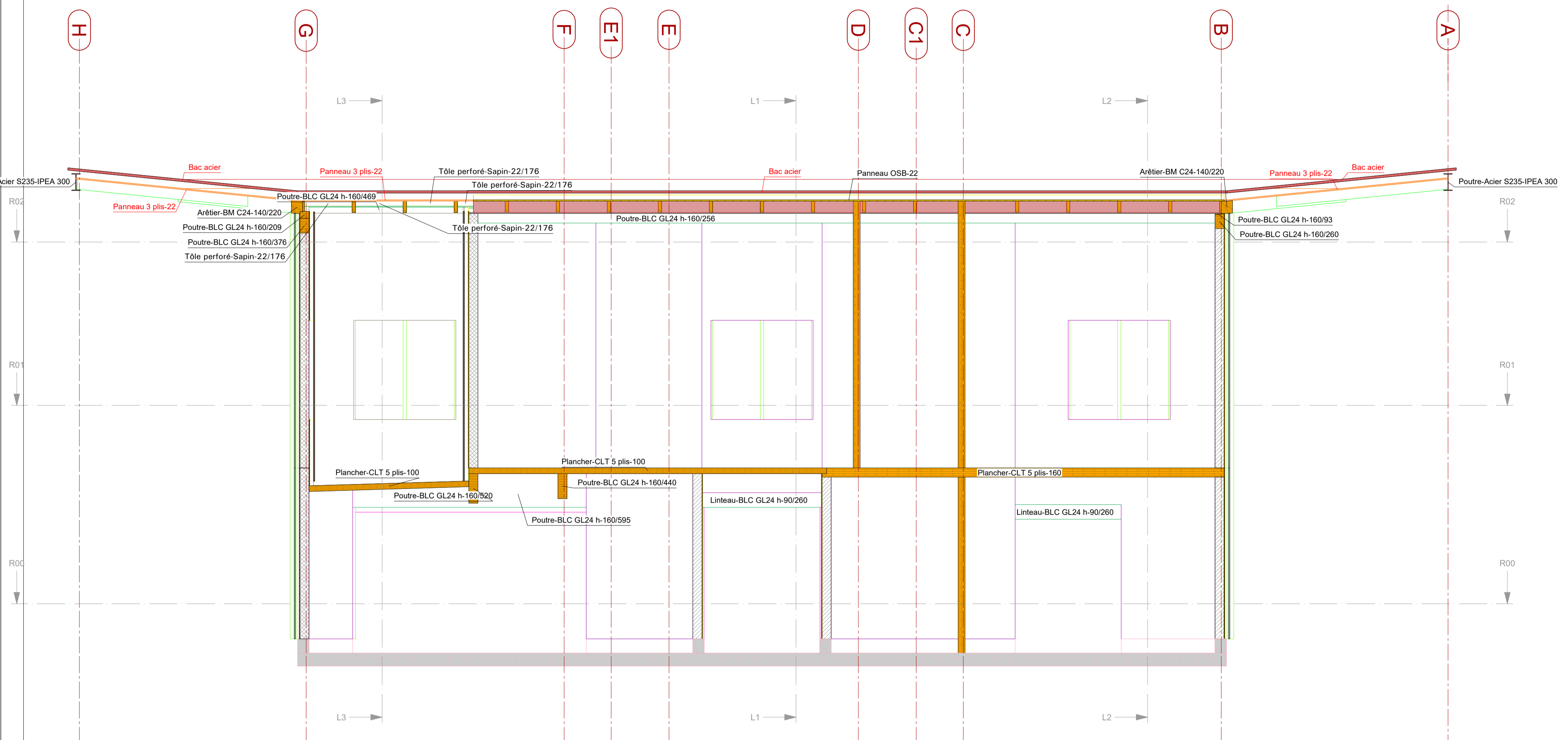
Coupe: T1-T1
