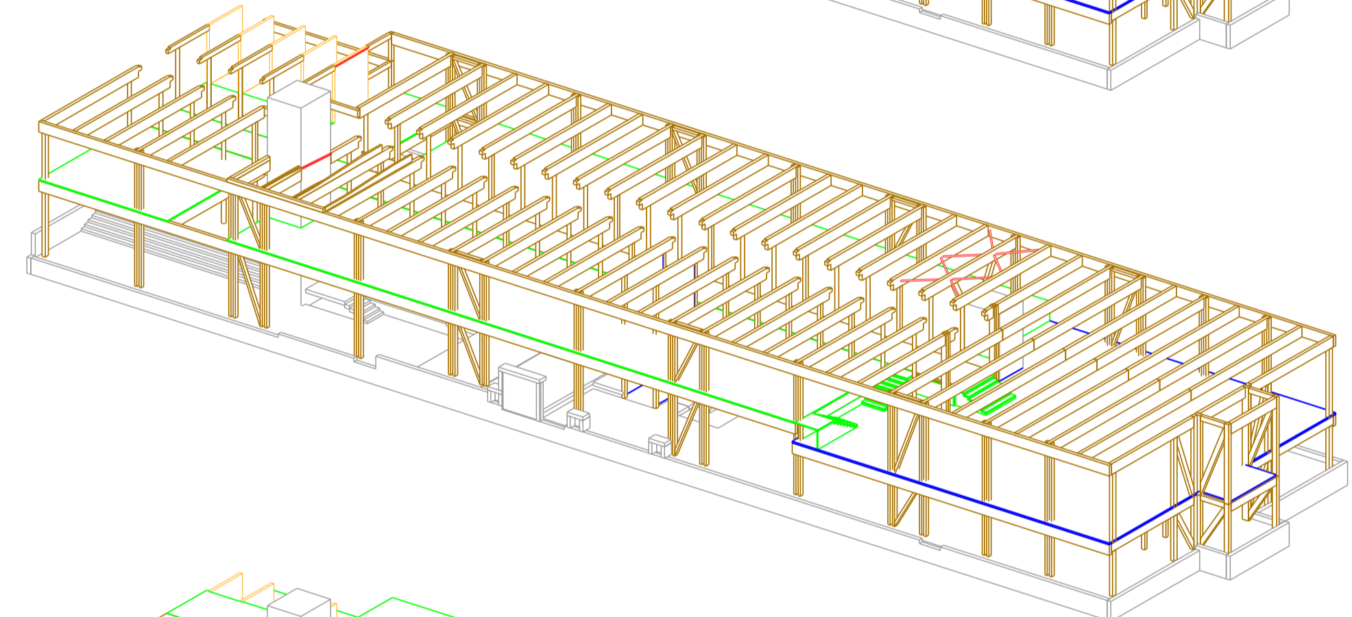
Structure bois R+1
