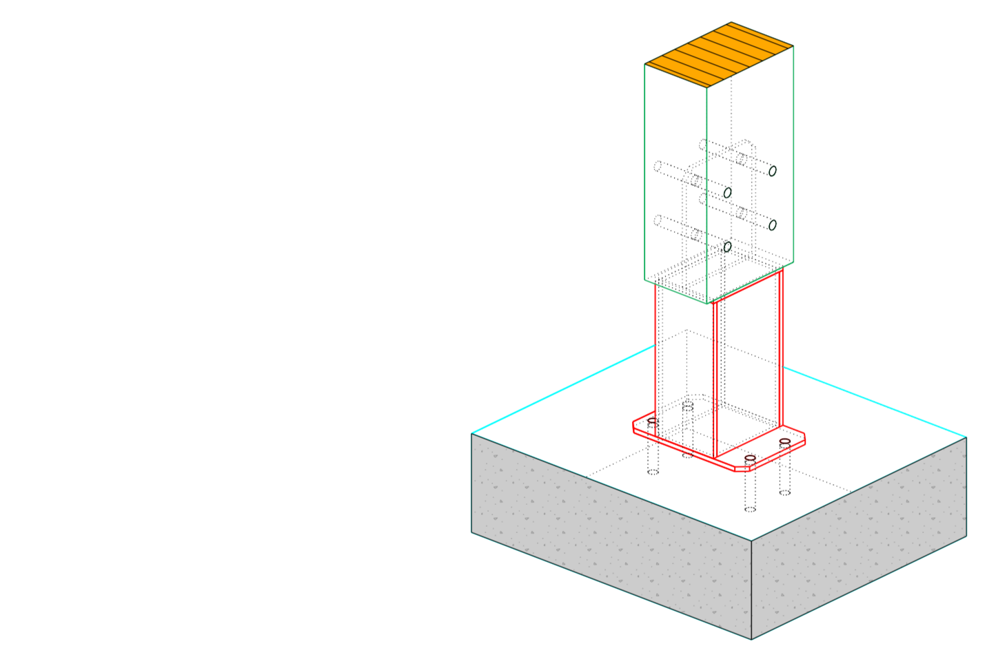
PRINCIPE PIED DE POTEAU BLC 160/250
