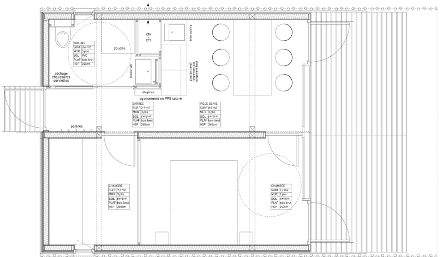
Plan double
