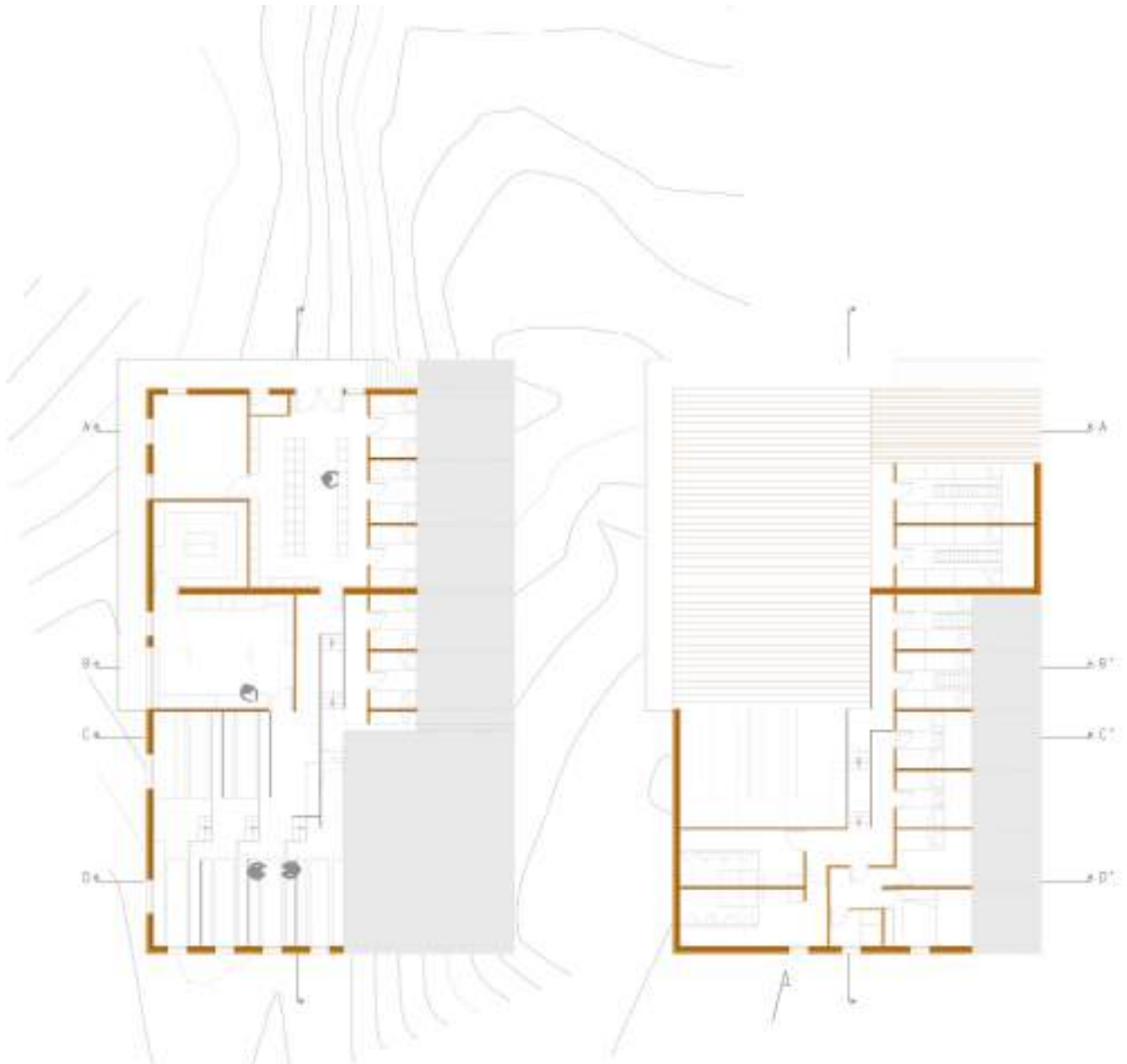
Plan rez-de-terre 1/100
