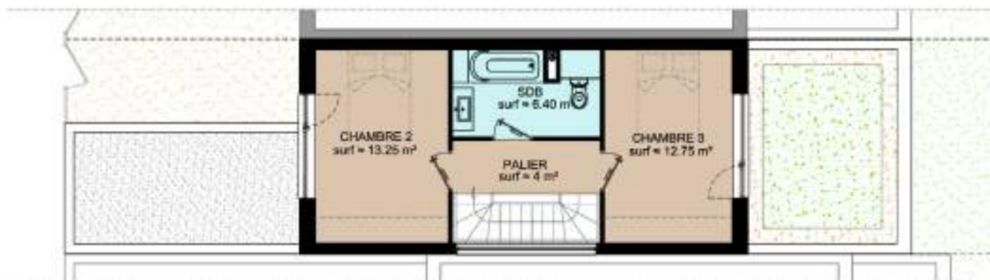
Plan 2ème Etage - Surface = 37 m 2
